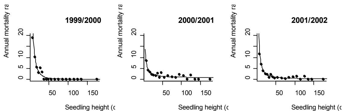
Figure 3. Annual rates of seedling mortality in relation to seedling height for mountain beech seedlings in three census years.
