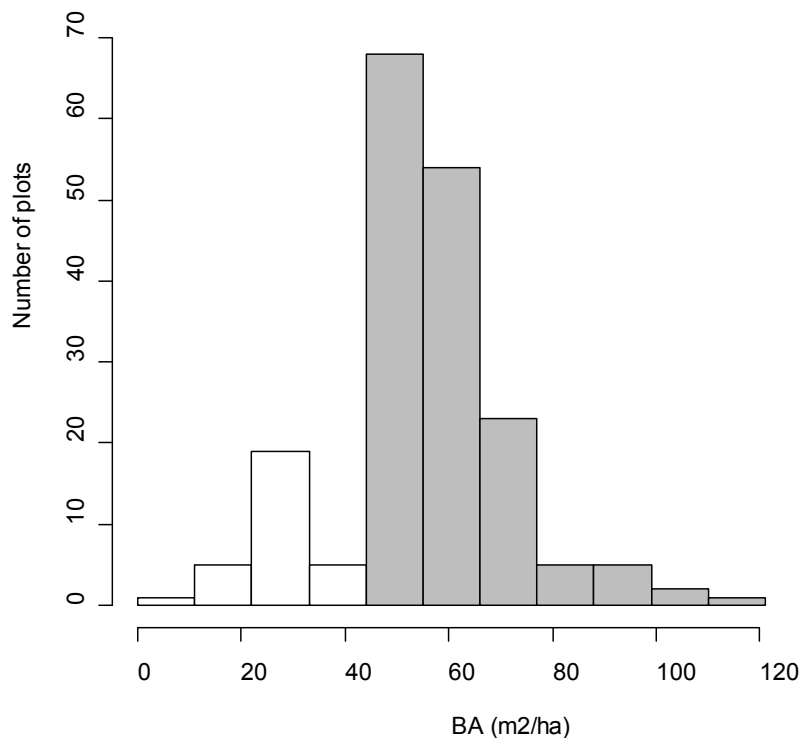
Figure 5. Frequency distribution of the basal area (BA) of the 189 mountain beech plots. BA <44 \text{ m}^2/\text{ha} shown as open bars; BA \geq 44 \text{ m}^2/\text{ha} shaded.
