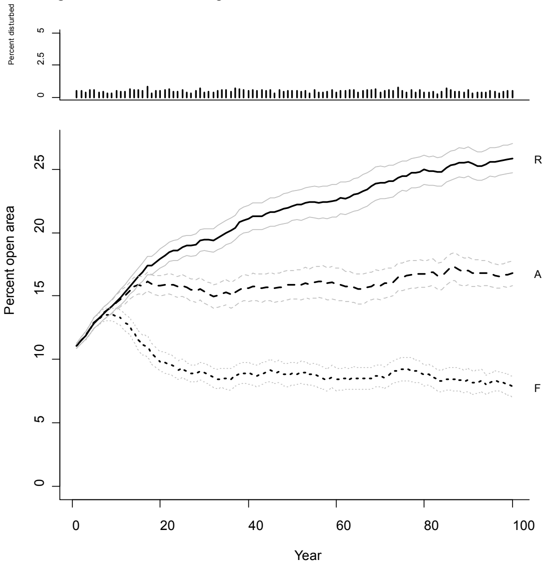
Figure 13. Averages from 100 runs of the simulation model. The upper graph shows the average percent of forest disturbed each year. The lower graph shows the corresponding average amount of forest in an ‘open’ state under each of the three deer control treatments, along with 95% confidence intervals around the means. R = recreational hunting, A = aerial hunting, F = fenced.
