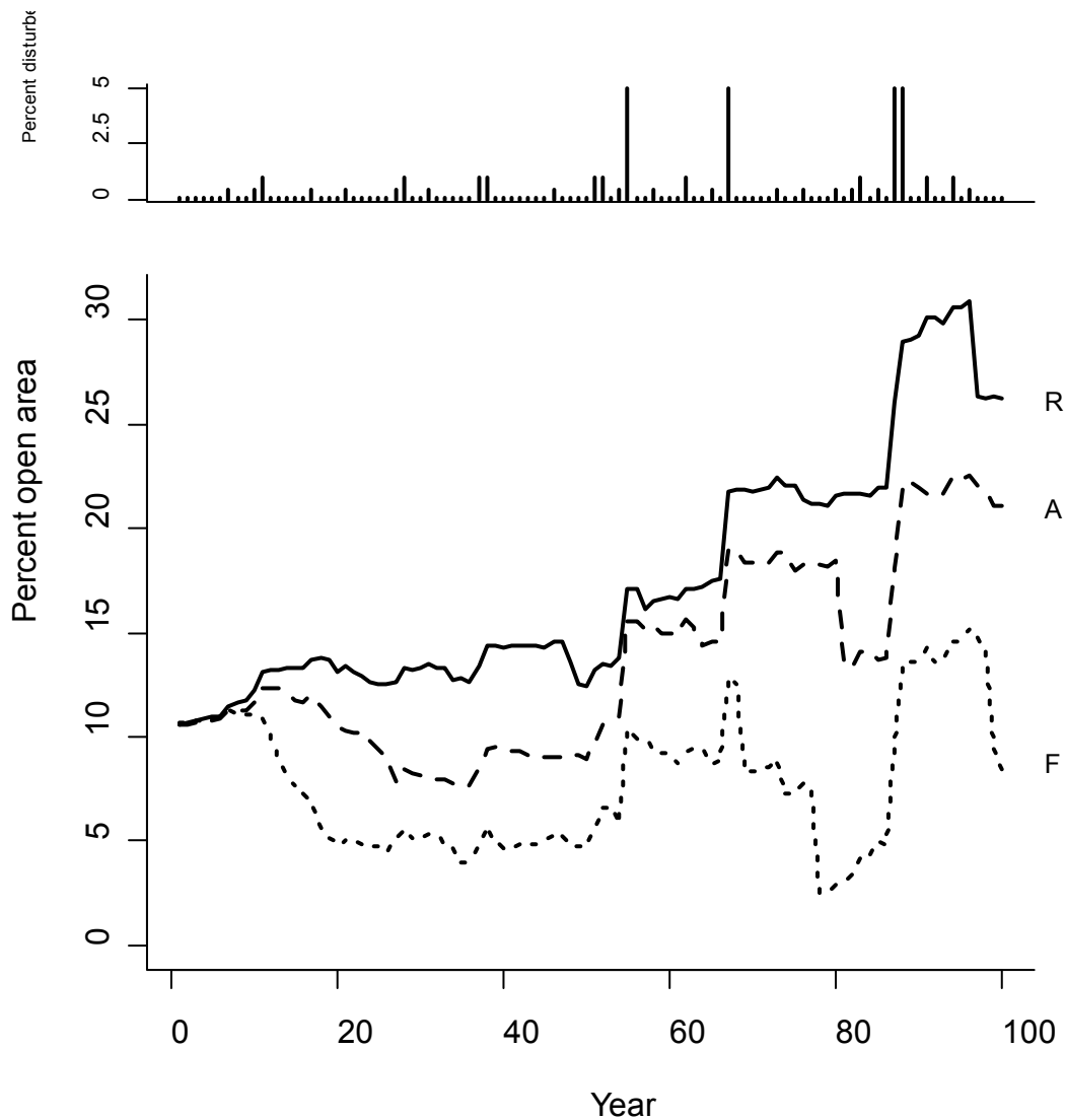
Figure 10. Result from a single 100 year run of the simulation model. The upper graph shows the percent of forest disturbed each year. The lower graph shows the corresponding amount of forest in an ‘open’ state under each of the three deer control treatments. R = recreational hunting, A = aerial hunting, F = fenced.
