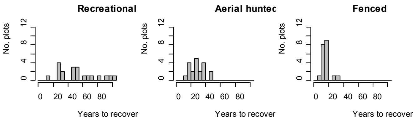
Figure 7. Frequency histograms of the time taken for each of the 20 plots to obtain an adequate number of stems >1.35 m in height under recreational hunting, aerial hunting, and fencing. Note that under recreational hunting, some plots failed to reach the minimum number of seedlings after 100 years. For these plots, 100 years is the minimum recovery time.
