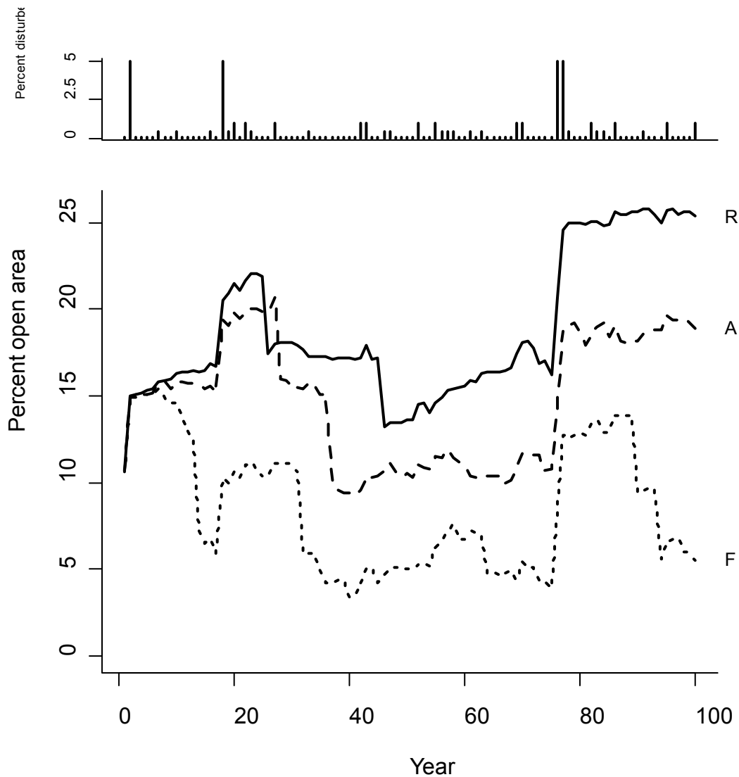
Figure 11. Result from a single 100 year run of the simulation model. The upper graph shows the percent of forest disturbed each year. The lower graph shows the corresponding amount of forest in an ‘open’ state under each of the three deer control treatments. R = recreational hunting, A = aerial hunting, F = fenced.
