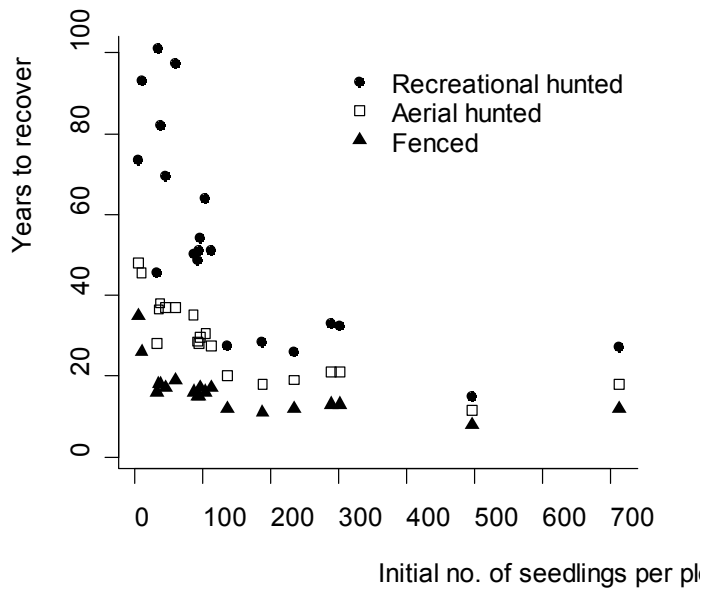
Figure 8. Relationship between initial seedling abundance on a plot and the time taken for that plot to recover under three levels of deer-control.
