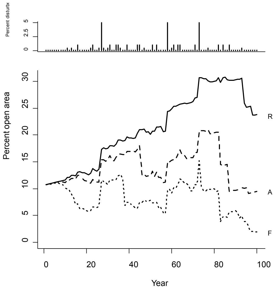
Figure 12. Result from a single 100 year run of the simulation model. The upper graph shows the percent of forest disturbed each year. The lower graph shows the corresponding amount of forest in an ‘open’ state under each of the three deer control treatments. R = recreational hunting, A = aerial hunting, F = fenced.
