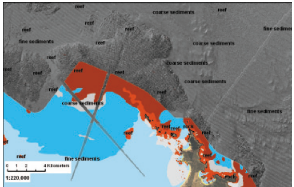
Figure 5c. Example of Ocean 20/20 multibeam sonar derived data layers— backscatter image draped over digital terrain model (Mitchell et al. , 2009). The area pictured is extending offshore to the northeast from Cape Karikari.
