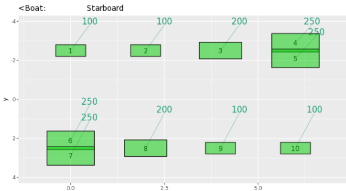
Figure 2 The configuration of the 1,800 CUI acoustic source array
