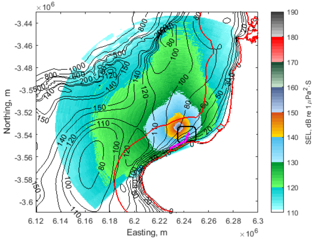
Figure 20 Maximum SELs predicted from the source location to a maximum range of 100 km overlaid with bathymetry lines
