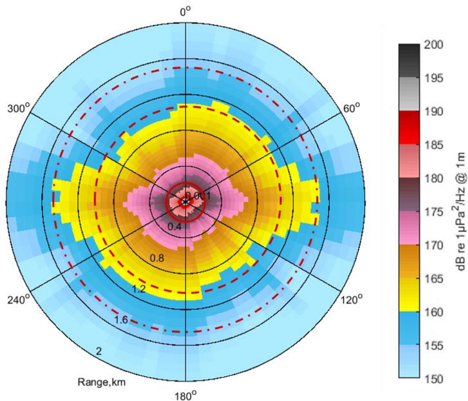
Figure 18 Predicted maximum received SELs across the water column as a function of azimuth and range from the centre of the 1,800 in 3 total source volume
