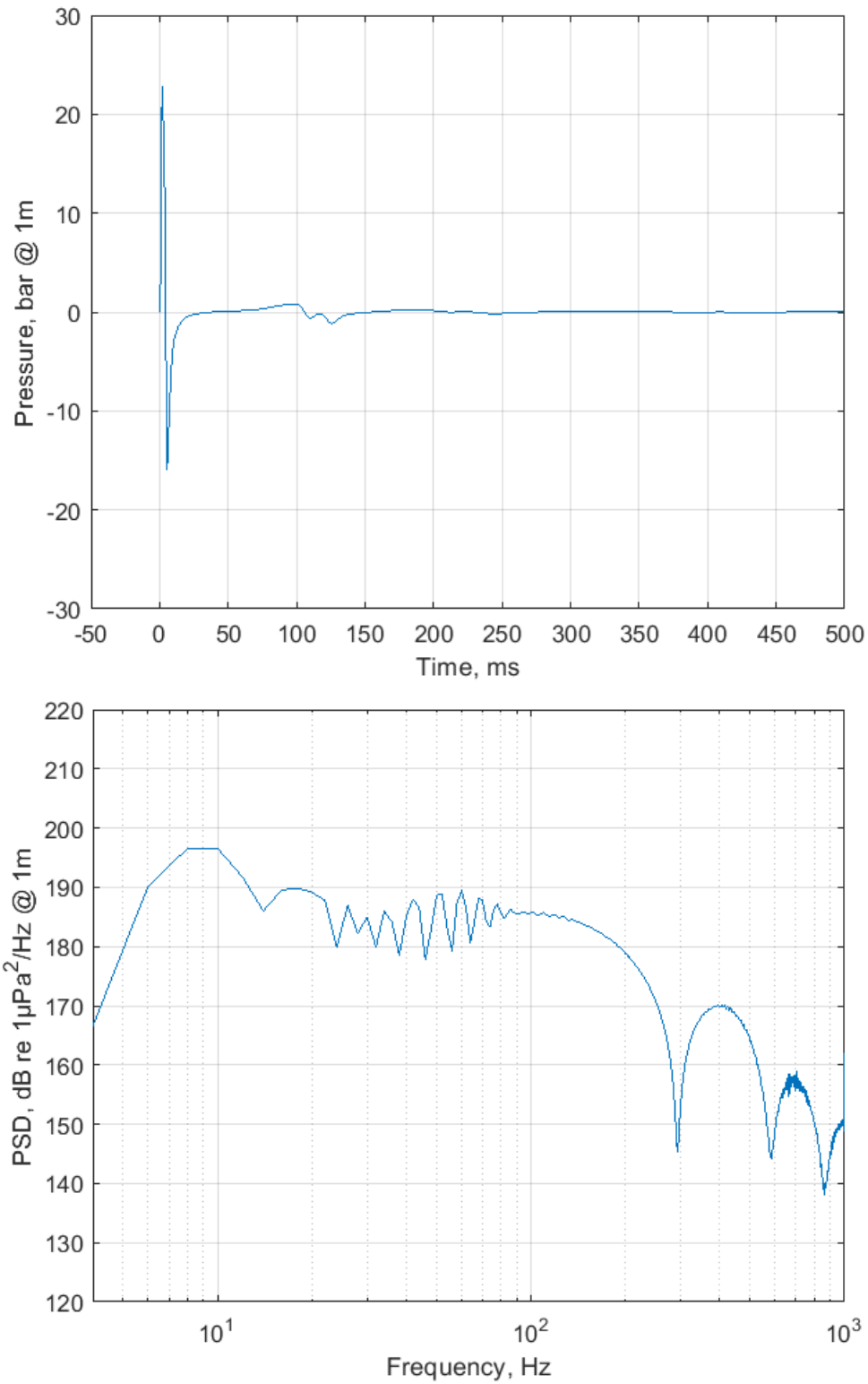
Figure 4 The far-field signature in vertically downward direction (top) and its power spectral density (bottom) for the 1,800 CUI array
