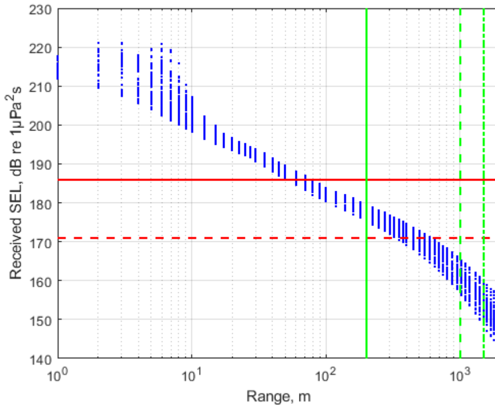
Figure 13 Predicted SELs across the water column for all azimuths as a function of range from the centre of the source array for the 1,800 CUI array at source location S1. Horizontal red lines show mitigation thresholds of 186 dB re 1\mu\text{Pa}^2\cdot\text{s} (solid) and 171dB re 1\mu\text{Pa}^2\cdot\text{s} (dash). Vertical green lines show mitigation ranges of 200 m (solid), 1 km (dash) and 1.5 km (dash-dot).
