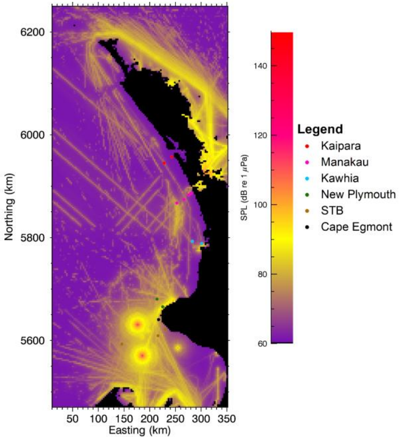
Figure 23 One- month equivalent continuous underwater noise levels ( L_{eq} ) for March 2015: high frequency weighted SPL
