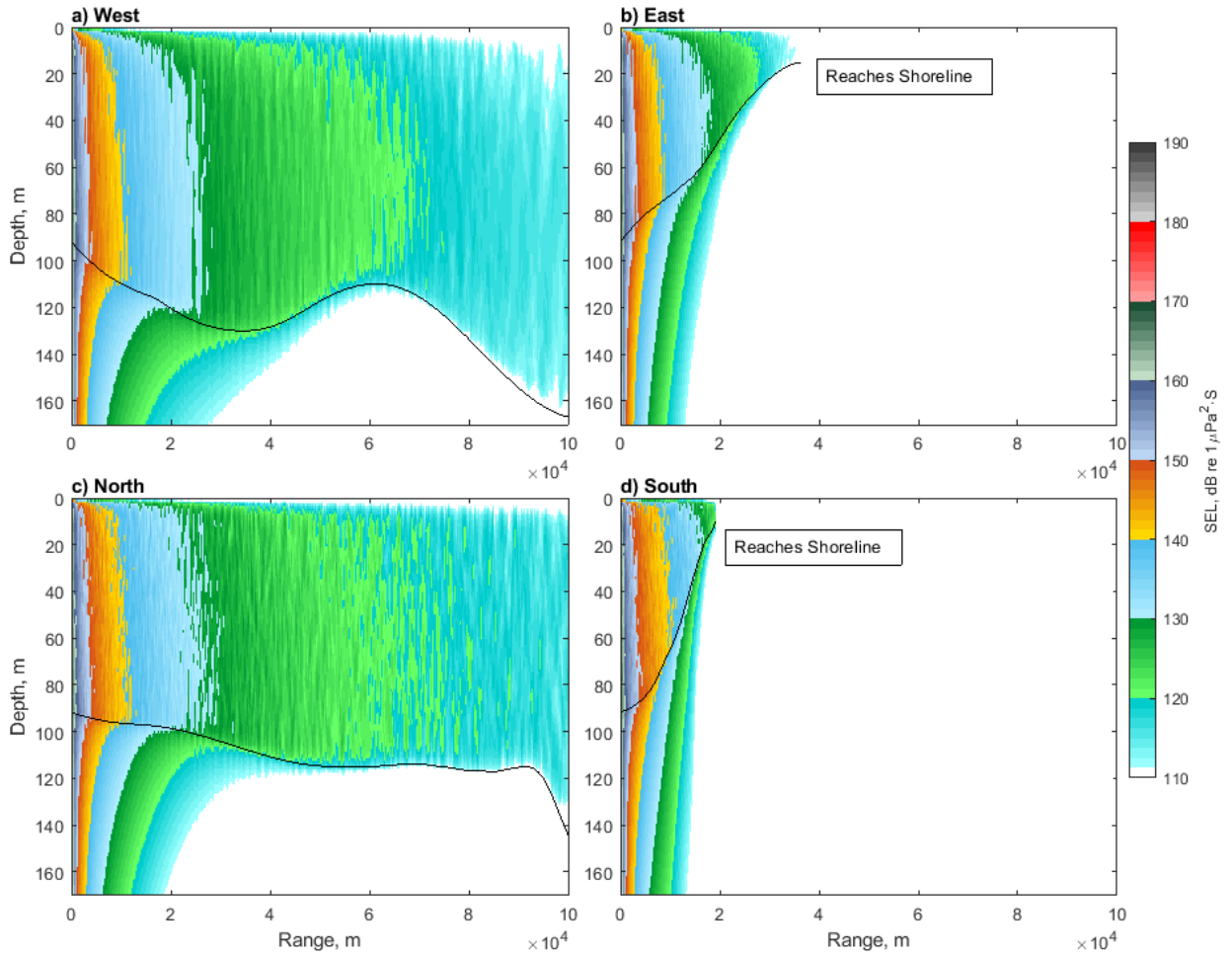
Figure 15 Modelled SELs vs range and depth along the propagation path towards a) west b) east c) north and d) south direction for the 1,800 CUI source array. The black line shows the seabed depth.
