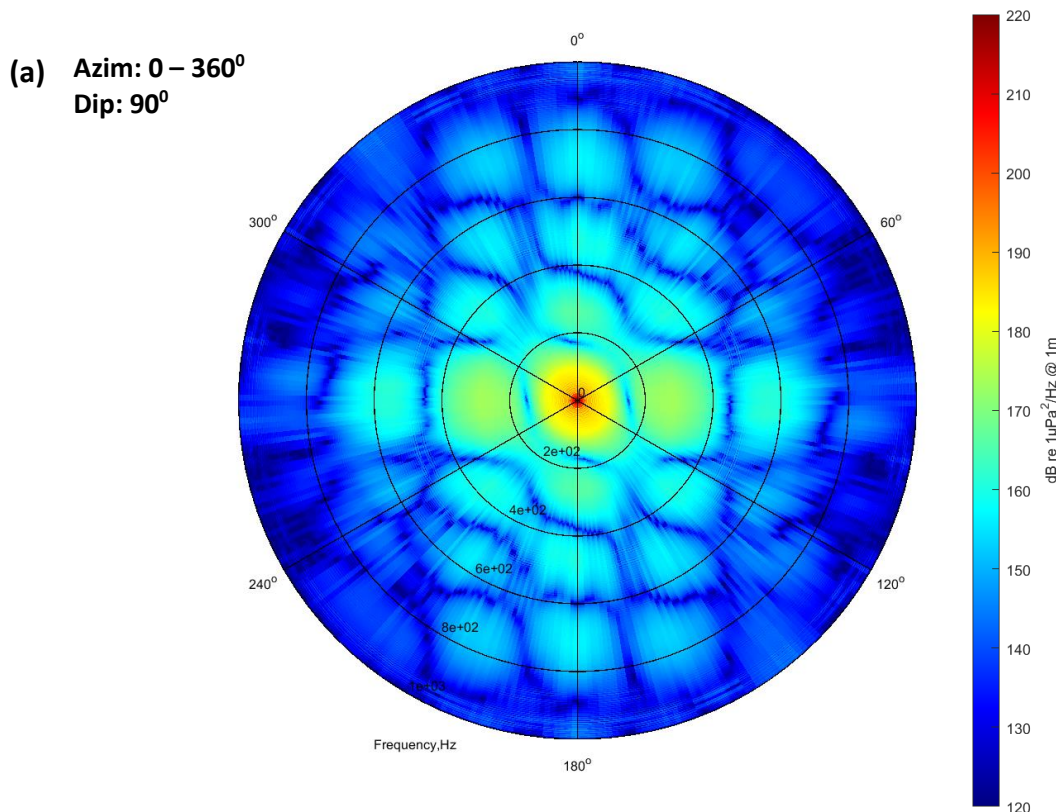
Figure 5 Array far-field beam patterns for the 1,800 CUI source array, as a function of orientation and frequency. (a) - The horizontal plane with 0 degree corresponding to the in-line direction; (b) – The vertical plane for the in-line direction; (c) – The vertical plane for the cross-line direction. 0 degree dip angle corresponds to vertically downward direction
