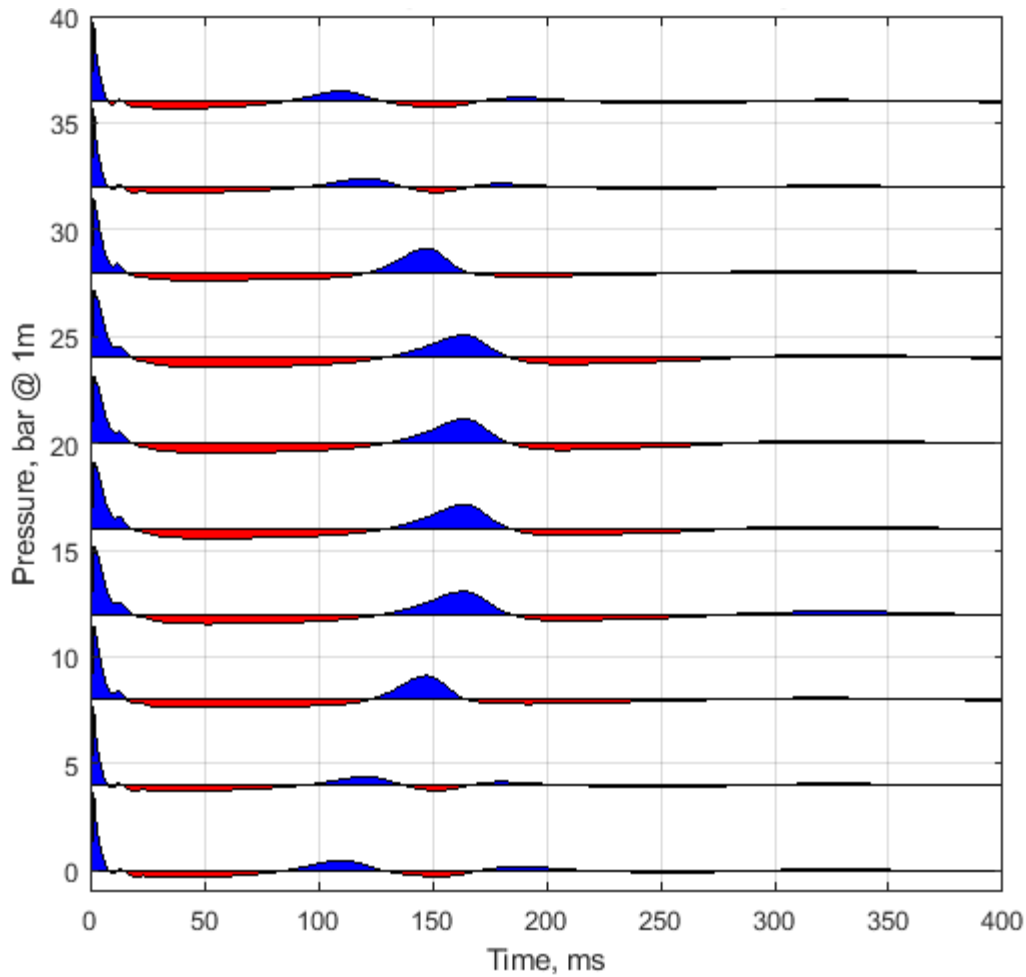
Figure 3 Notional source signatures for the 1,800 CUI acoustic source array
