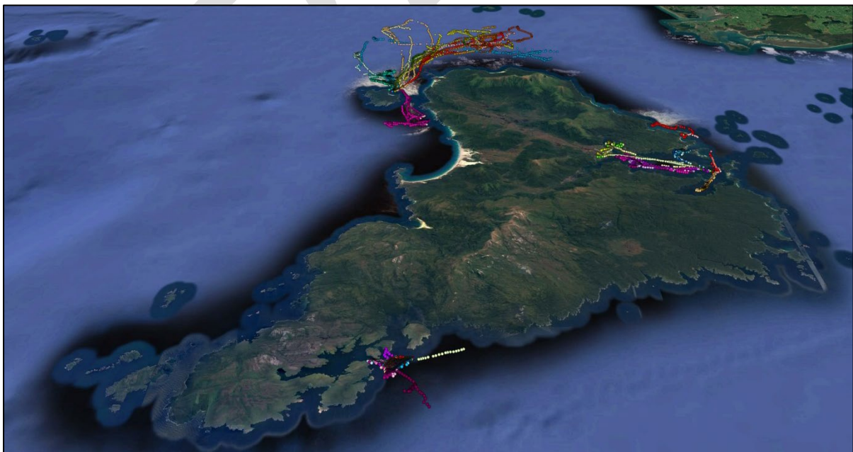
Figure 8. Overview of distribution of GPS data recorded during the chick rearing period 2020/21 at the three main study sites.
