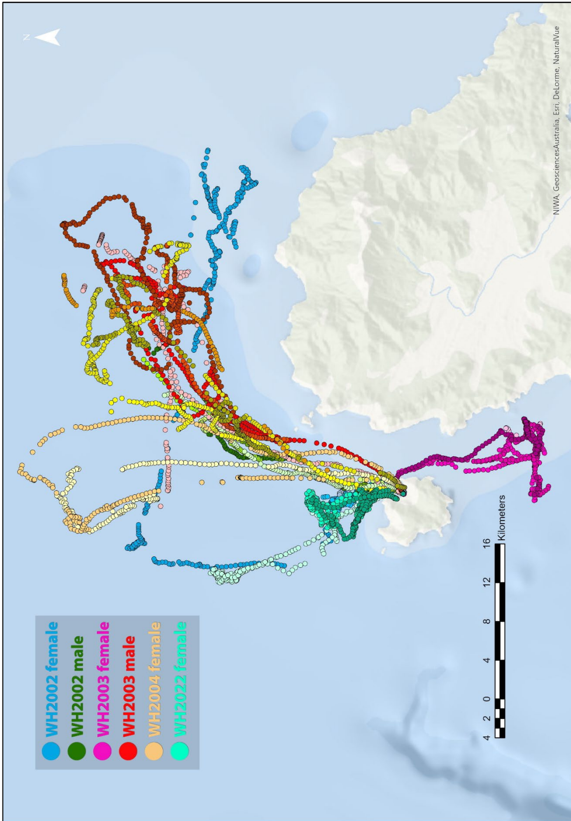
Figure 13. Overview of distribution of foraging locations in hoiho from Whenua Hou post-guard stage of the 2020/21 season (January 2021).
