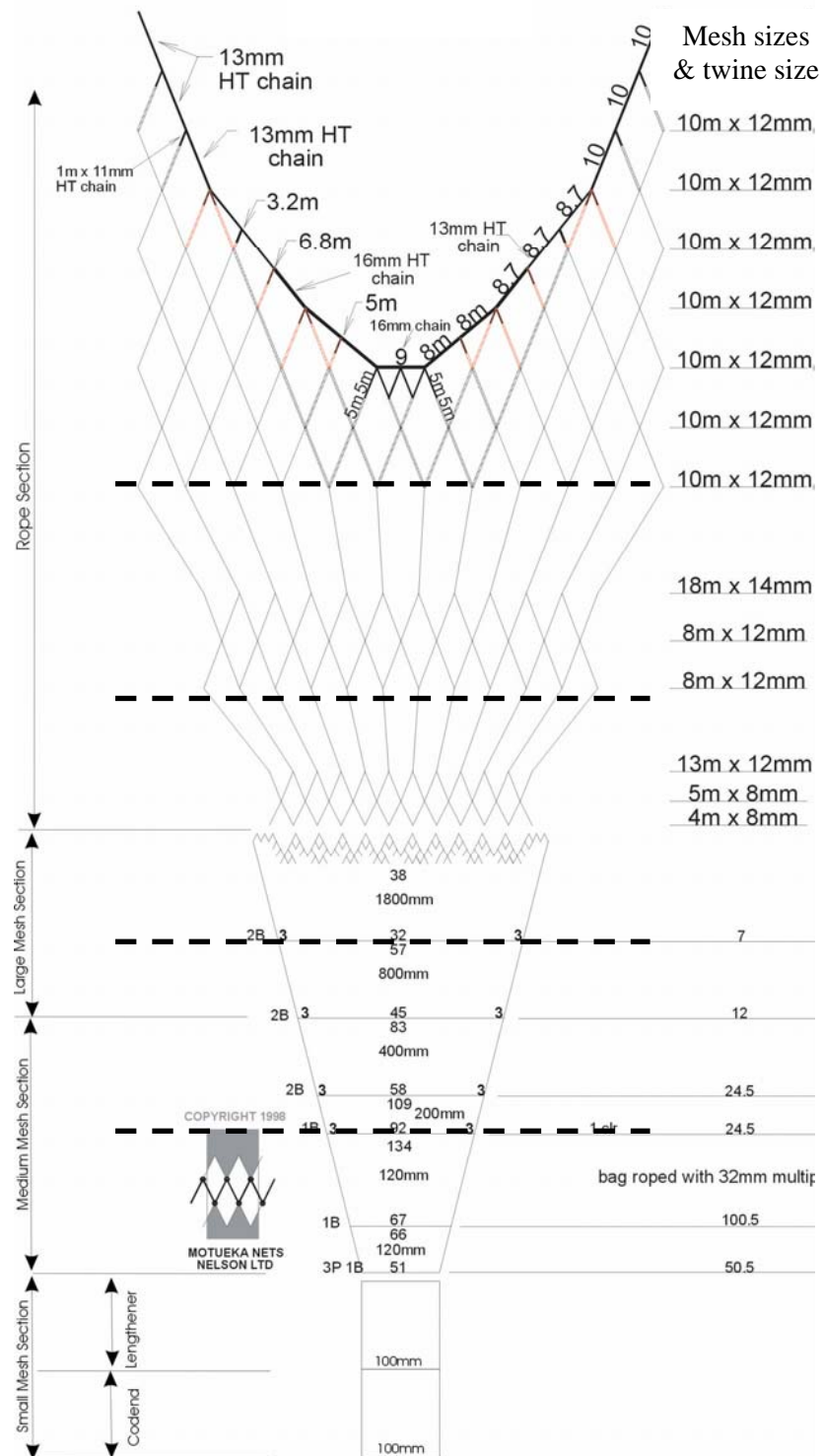
Figure 10: Dashed lines show initial positions of ties for the net binding trial
