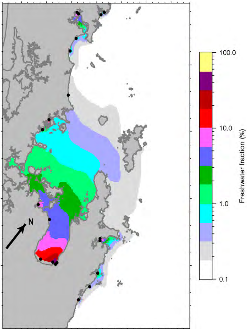
Figure 6: Time-mean surface freshwater concentration from the Hauraki Gulf model. The mean is evaluated over a two-year period ( t = 170 d to t = 900 d) for the simulation described in Section 3.4. Note the log10 colour scale.
