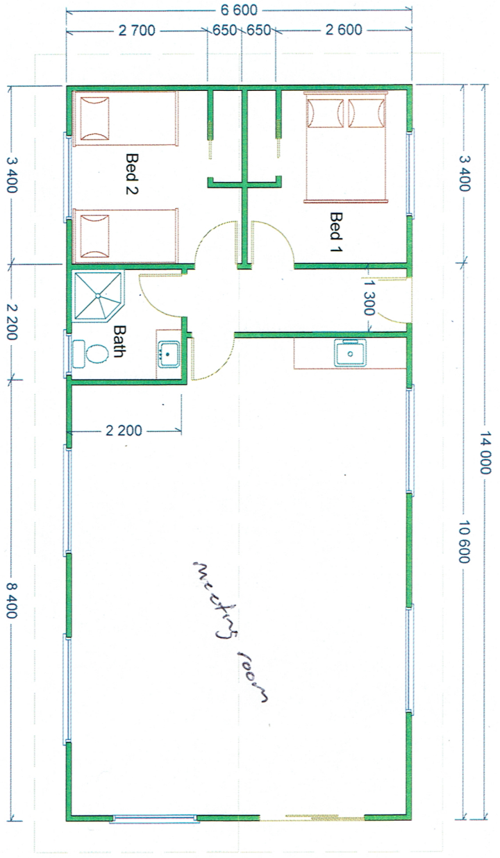
Timber Trail Staff/meeting room Floor Plan Scale 1:100
